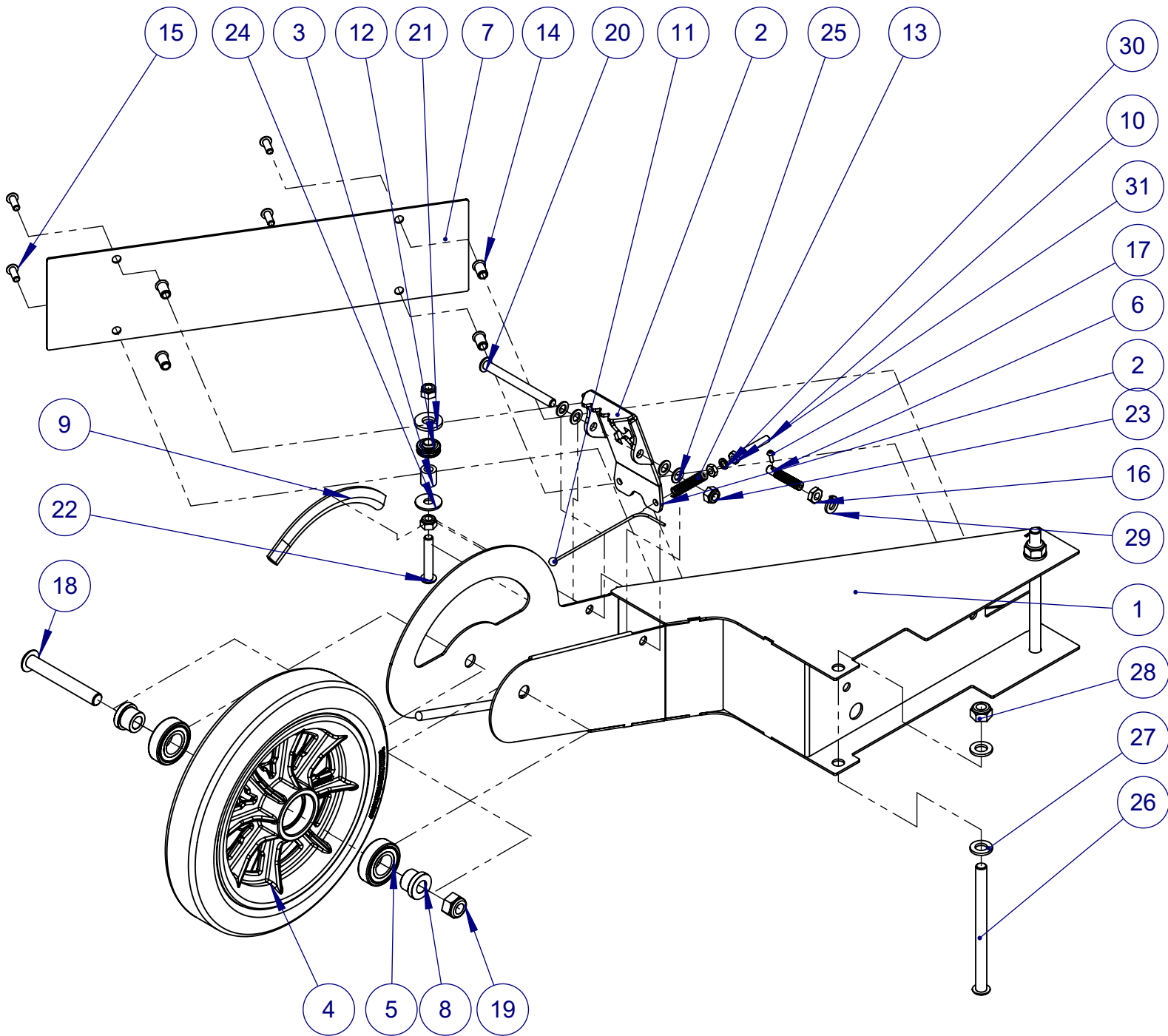
EXPLODED VIEW
