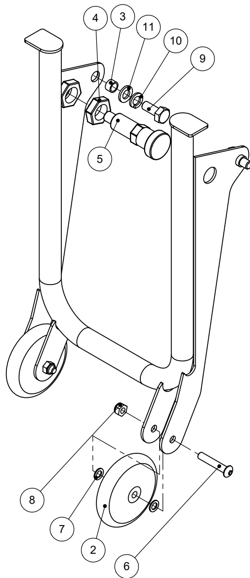
EXPLODED VIEW
