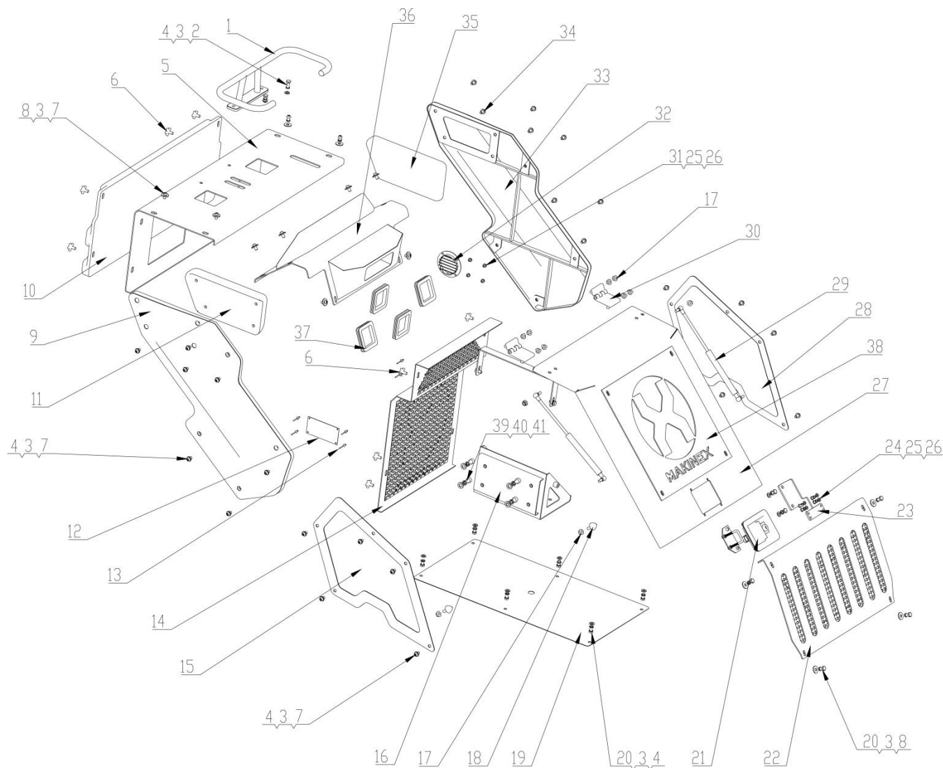
Exploded Diagram 6
