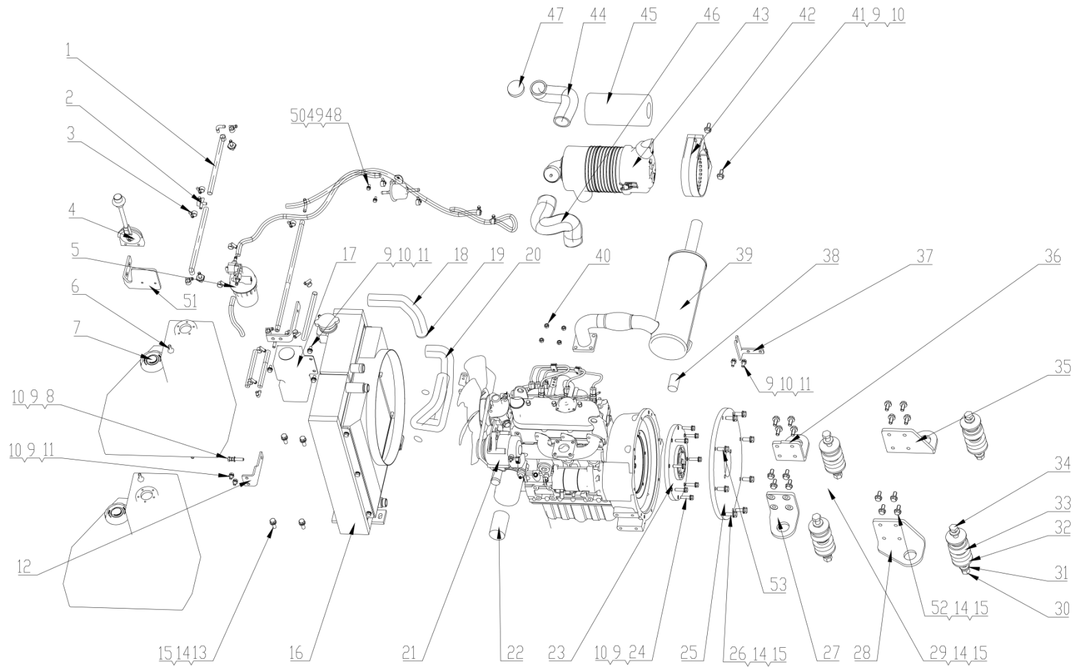
Exploded Diagram 3
