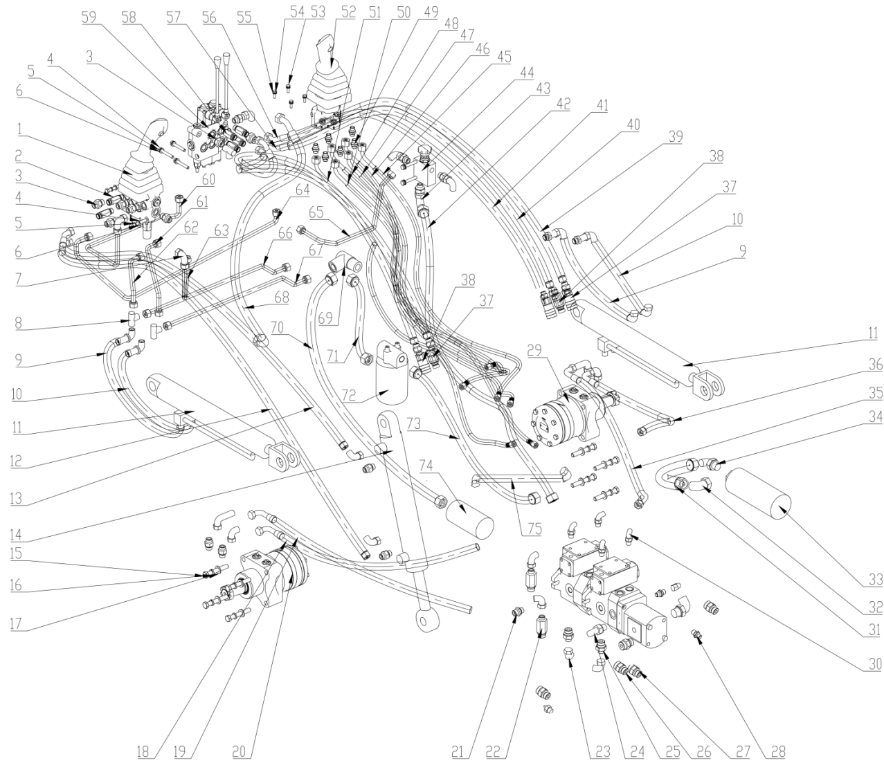
Exploded Diagram 4
