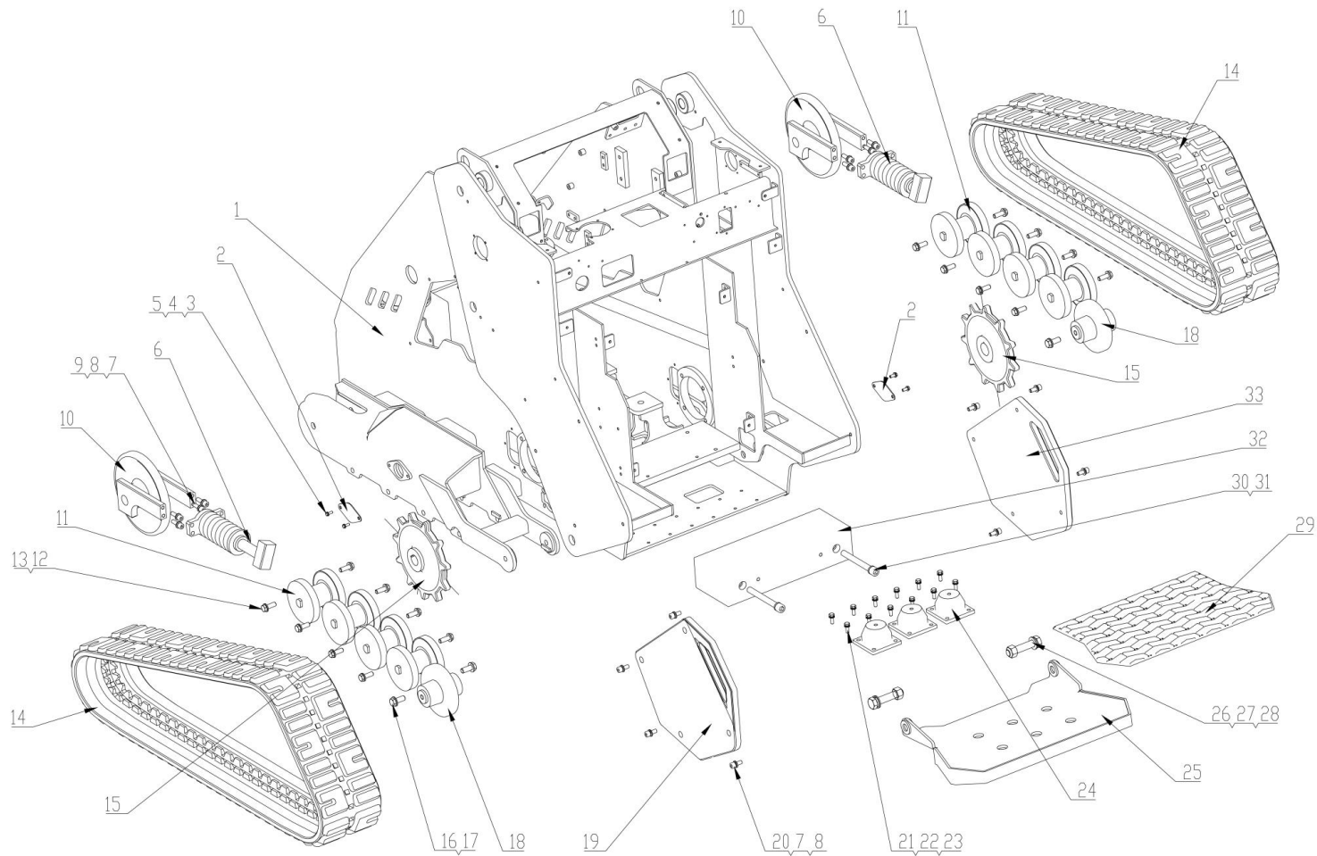
Exploded Diagram 1
