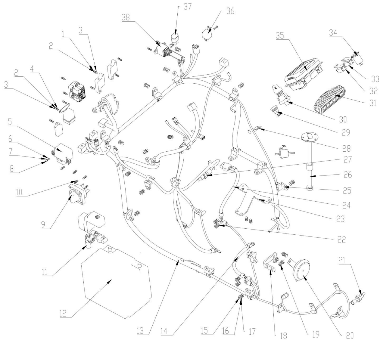
Exploded Diagram 5
