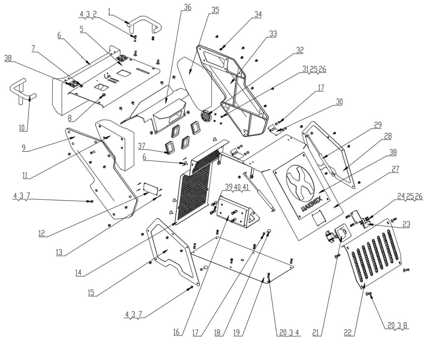
Exploded Diagram 6
