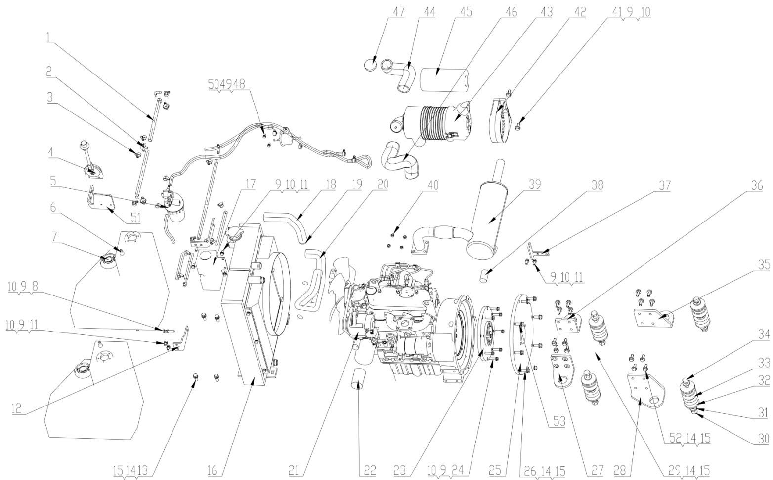
Exploded Diagram 3
