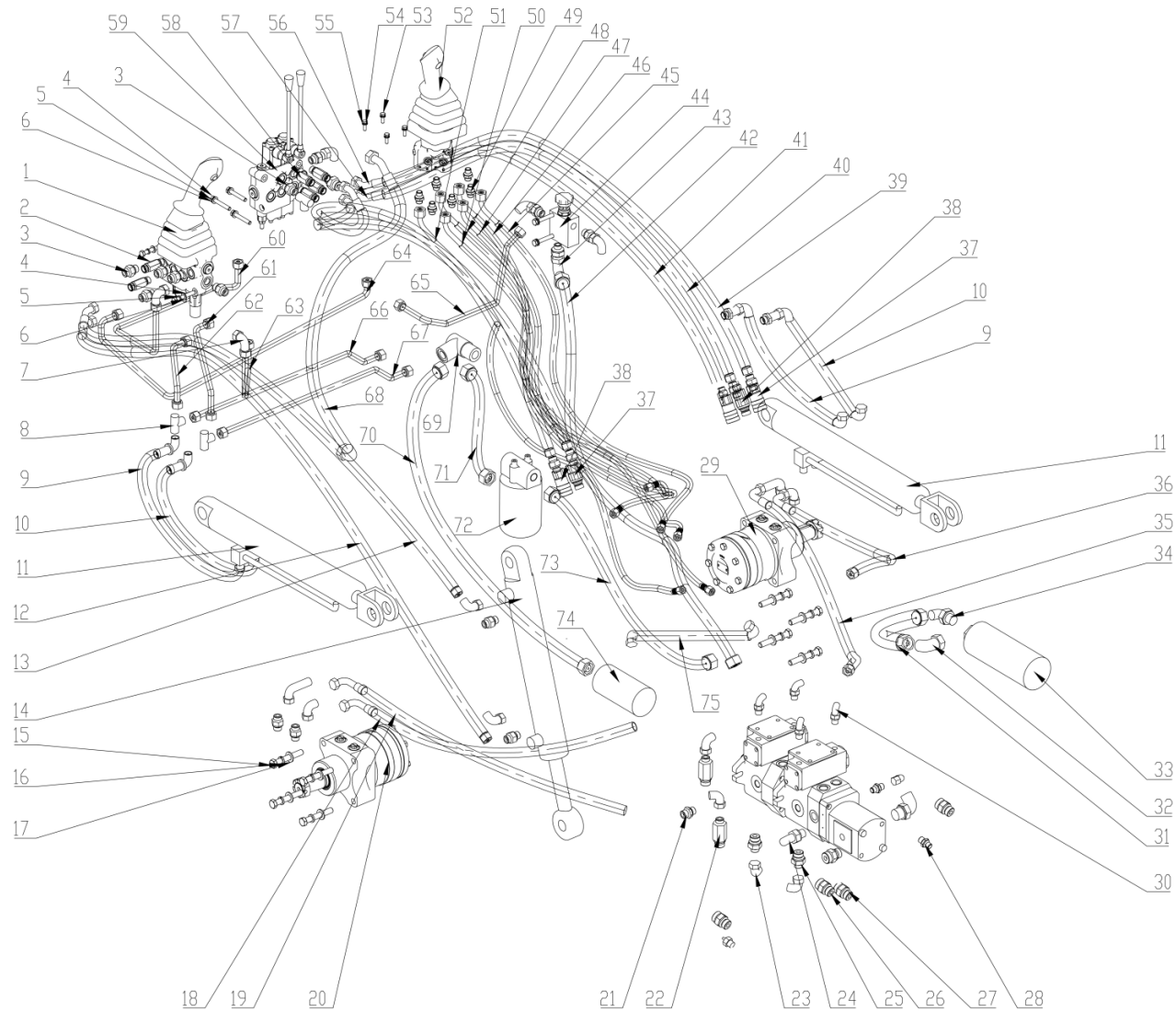
Exploded Diagram 4
