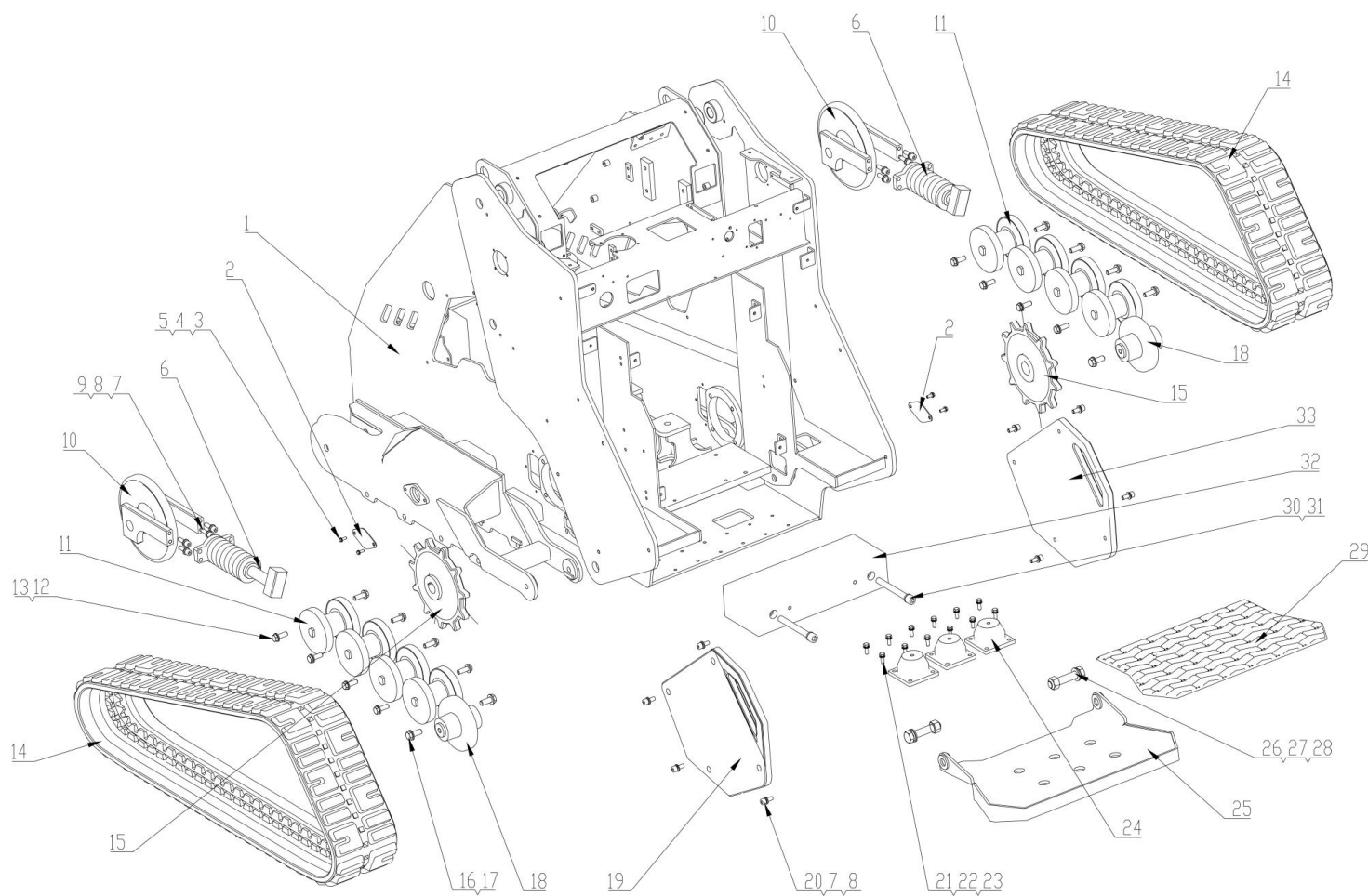
Exploded Diagram 1
