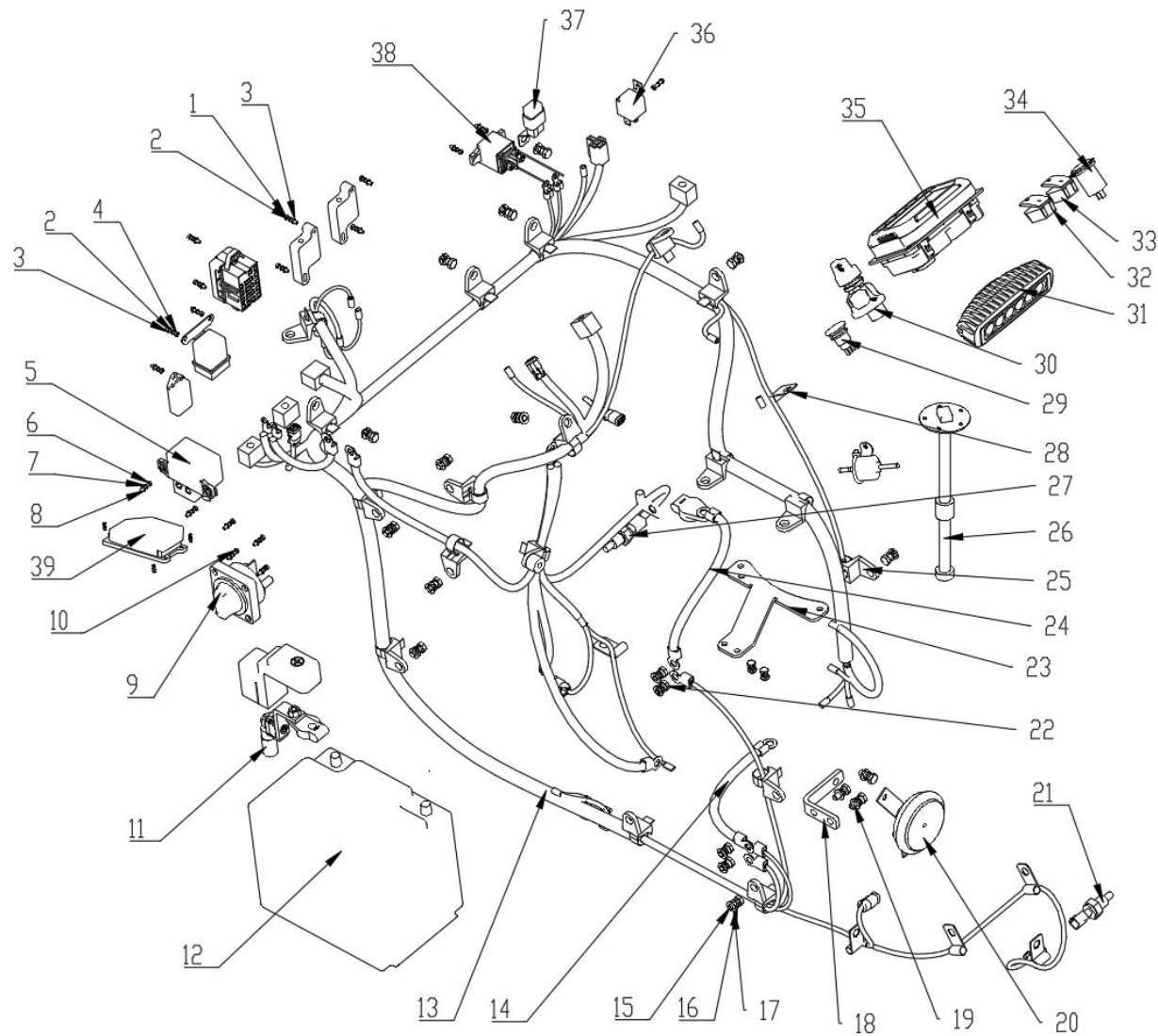
Exploded Diagram 5
