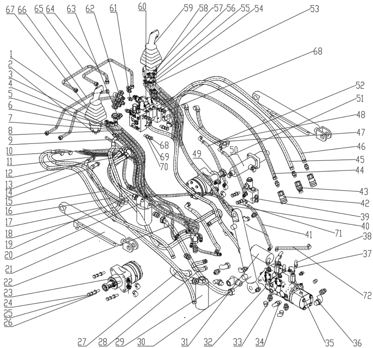
Exploded Diagram 4
